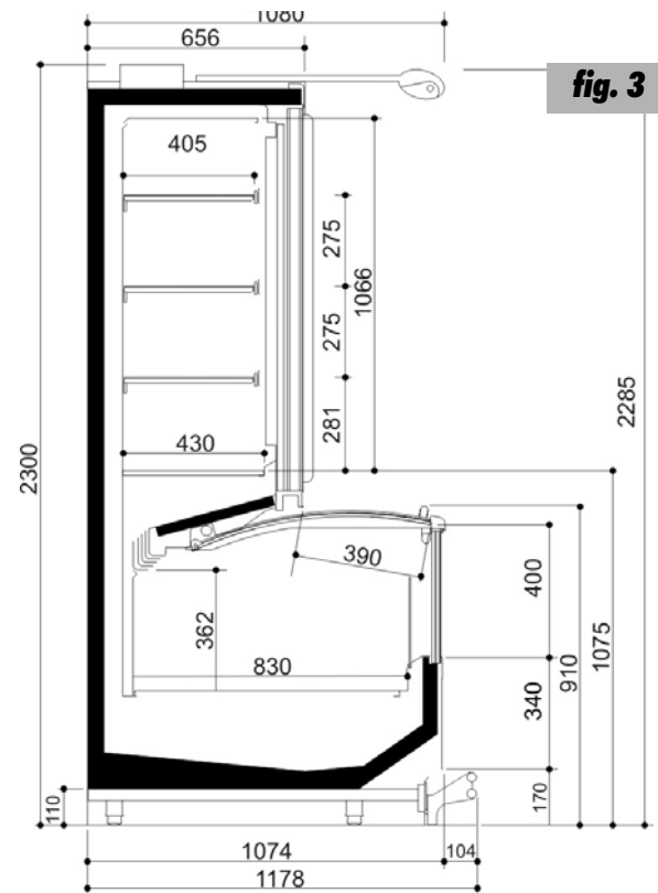
COLISUEM 4 ECO H2200
