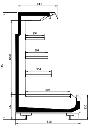
NordicStar SV5 30-89-165
