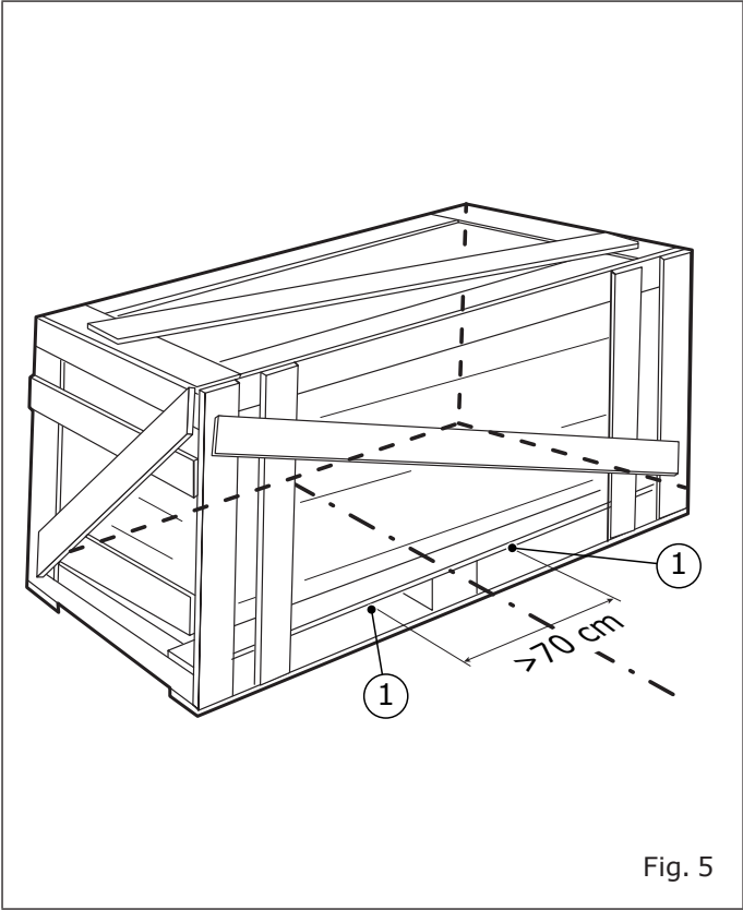
1. Lifting points
