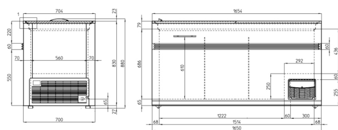
SLIDING_GLASS
