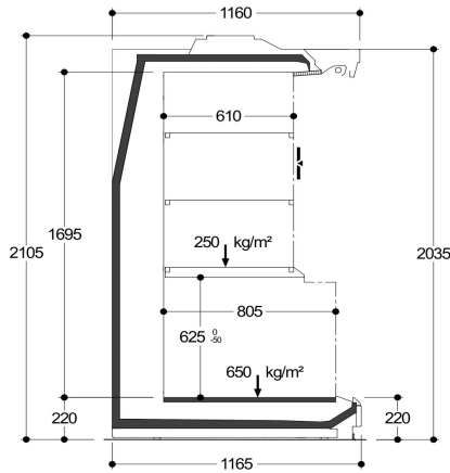
HD8 20 L Cross Section
