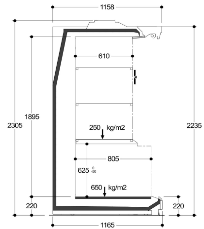
HD8 22 L Cross Section
