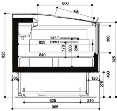
EOL - DUAL
