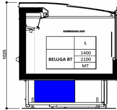
EPTABLUE - OPTION
