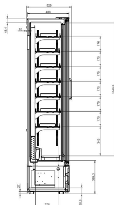
MULTITINY PLUS
