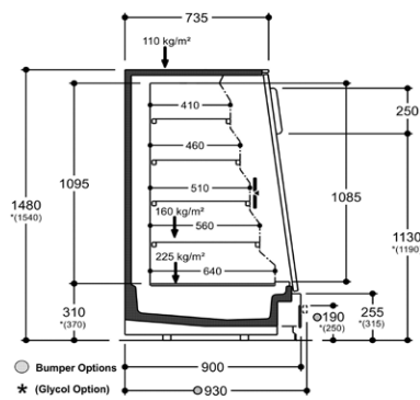
MODULAR - H15 TILTED DOORS
