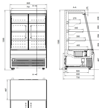
SV8 PI 90 140 C GD (3 shelves) Closed
