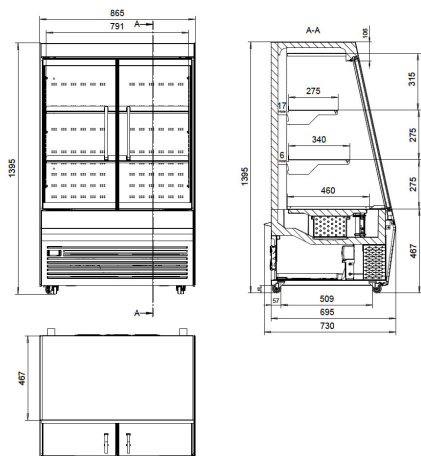
SV8 PI 90 140 C GD (2 shelves) Closed
