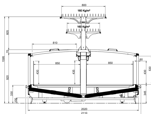
GRANONTARIO SLIDING 2 SHELVES
