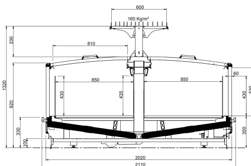
GRANONTARIO SLIDING 1 SHELF
