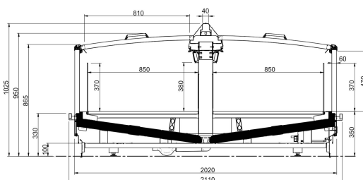
GRANONTARIO LARGE ERGO SLIDING COVERS LINEAR
