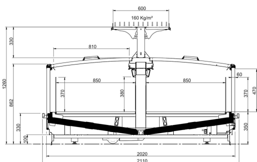
GRANONTARIO LARGE ERGO - SLIDING COVERS WITH SUPERSTRUCTURE 1S
