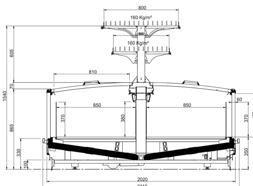
GRANONTARIO LARGE ERGO - SLIDING COVERS WITH SUPERSTRUCTURE 2S
