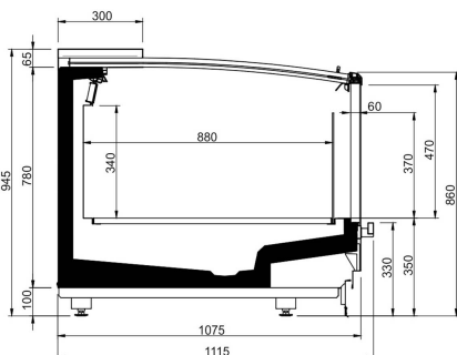
GRANDRAKE ERGO PUSH COVERS LINEAR
